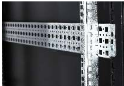
可前后调节的覆铝锌方孔条 The zincalume mounting profile could be adjustable
