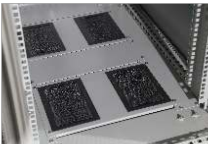
底板预制走线孔毛刷封闭 Sealing of prefabricated wiring holes on the bottom plate with brush
