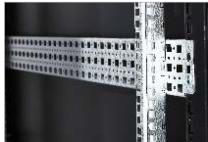
可前后调节的覆铝锌方孔条 The zincalume mounting profile could be adjustable
